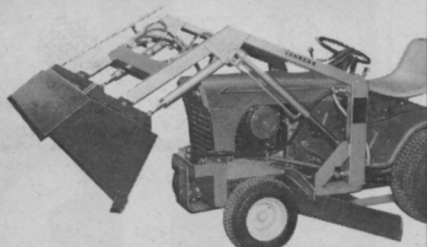
LOADER & TERRA-BLADE MOWER OR TERRA-BLADE MOUNT WITH LOADER ON MOST TRACTORS
