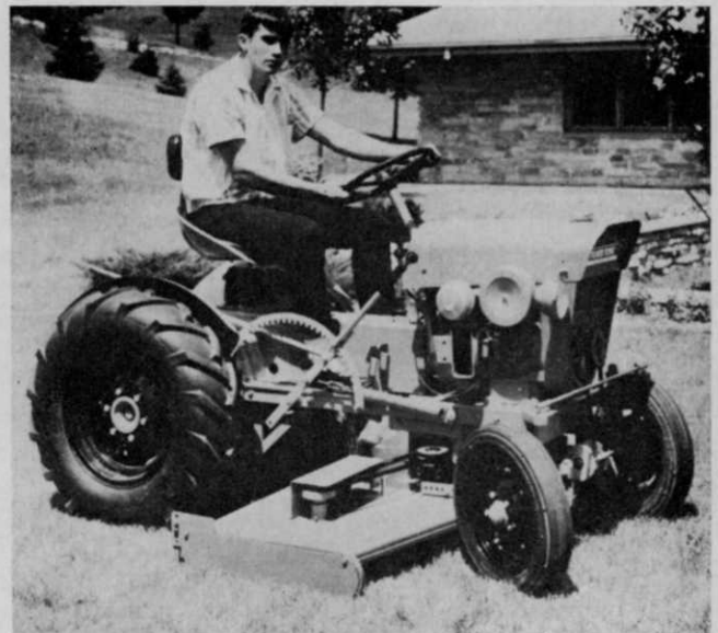
Economy tractor , below, handles rotary mowers up to 60 inches. Mows 3 acres per hour. Cutting height adjustment, foot operated clutch for disengaging cutting knives, lift mechanism for raising during travel, heavy cover, and sheave guards. Tractor has 12-hp engine, automotive drive train, welded frame, 16- and 24-inch wheels. Also handles 4-foot dozer blade, ¼-ton front end loader, 36- and 48-inch snow blowers and implements. Write Engineering Products Co., 1005-HF, Anoka Ave., Waukesha, Wis.
