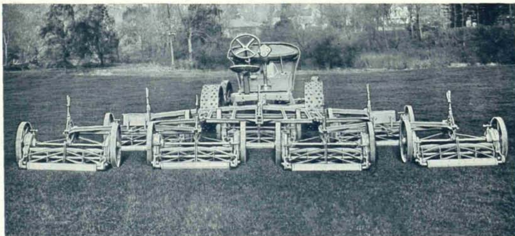
THE WORTHINGTON "CONVERTIBLE MULTIGANG"
