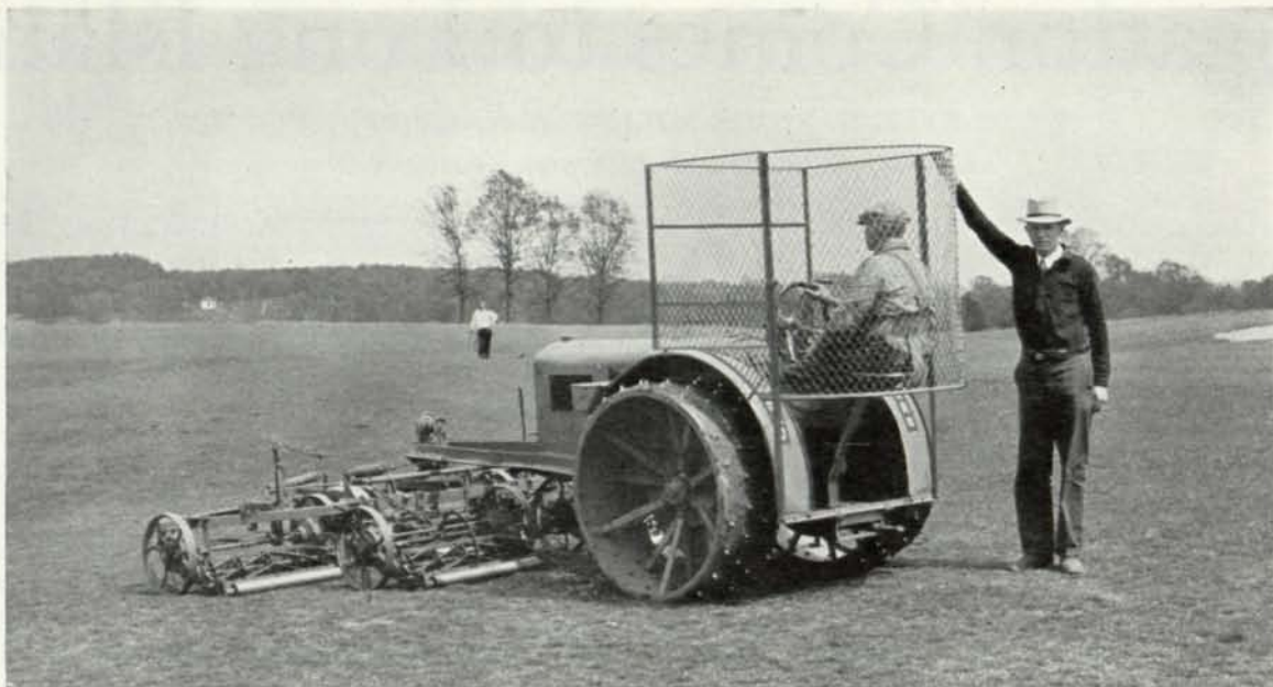
TORO TRACTOR WITH WIRE CAGE ENCLOSURE FOR THE OPERATOR This device is used by George Post, greenkeeper at Franconia Club, Springfield, Mass.
