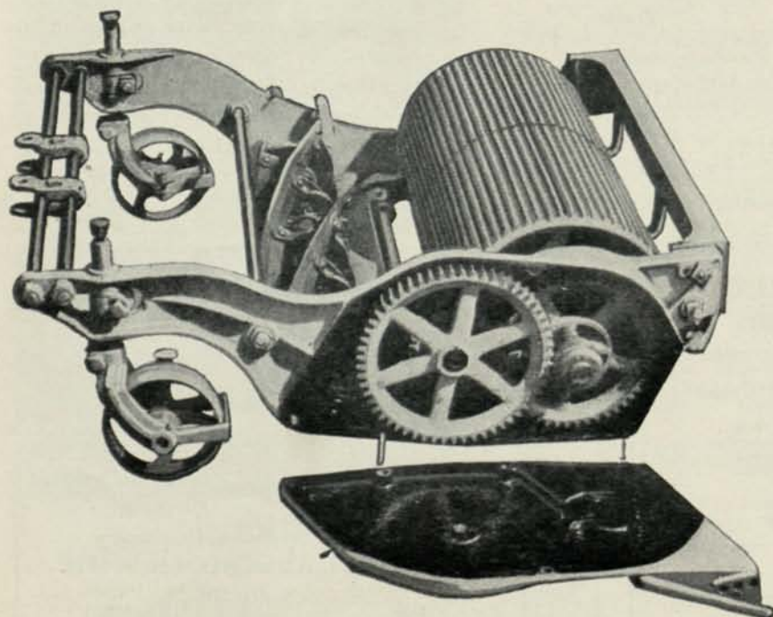
The Roseman Fairway Mower Carries a Roller Which Provides Traction and, So the Maker Claims, Produces Better Turf
