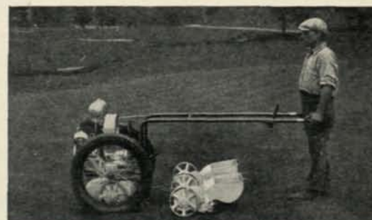
The "Overgreen" power putting green mower is making as great a revolution in the cutting of golf greens as the Worthington gang mower has made on the fairway. It will mow the 18 greens of the average course in four hours and one-half. It is guaranteed to leave the putting surface, in respect to smoothness and freedom from any mark, in unexcelled condition. Unequalled in durability and freedom from derangement or delays
