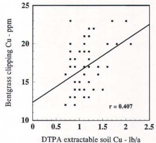
Figure 1. Relationship of DTPA extractable soil Cu to bentgrass clipping Cu concentration.
