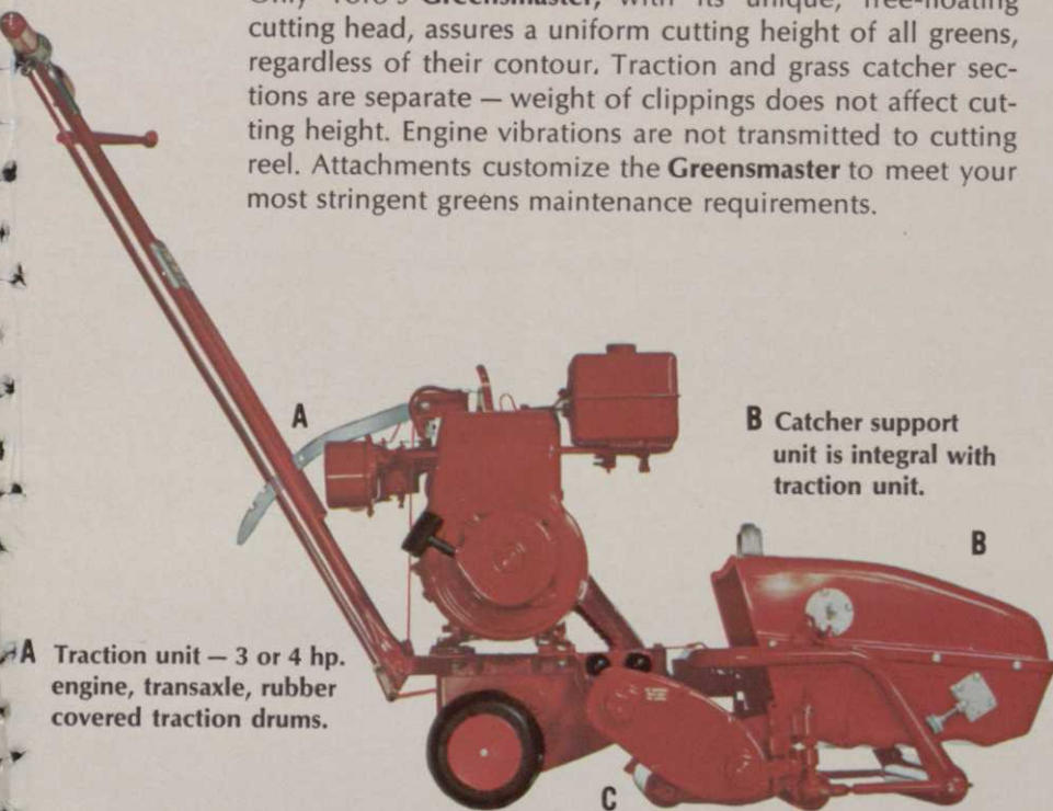
C Free floating cutting unit has 21", 9 blade reel.
