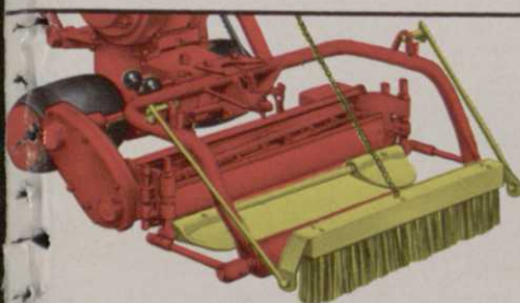
Brush Attachment easily adjusts for light or heavy brushing. Eliminates grain, assists in thatch control, lifts stringers.
