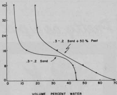
Fig. 2: Moisture content of 0.3-0.2 mm dia. sand and sand plus 50 per cent by volume of coarse spagnum peat as determined by height above water table.
