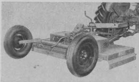
MODEL 80 (61 similar) with 80" cut, 2 blades for 2-3 plow tractors. Available with hand crank or hydraulic cylinder brackets for height adjustment.
