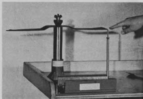
Model 10 Simplex Rotary Balancer, mfd. by Fate-Root-Heath Co., Plymouth, O., makes it possible for any serviceman to accurately balance and track any rotary blade mower with mounting holes \frac{3}{8} -in. to 1\frac{1}{2} -in. in diameter.
