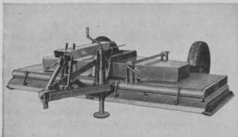
MODEL 114 with 114" cut, 3 blades, available with hand crank or hydraulic cylinder brackets for height adjustment.
