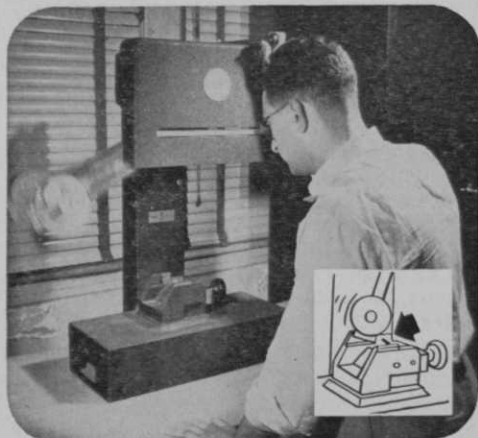
(Above) Impact test. Before approval can be given to production, raw material is tested for satisfactory resistance to impact. (Right) Tensile strength test. Virgin polyethylene is stretched to its limit to make sure Triangle Plastic Pipe will have more than its guaranteed working pressure.
