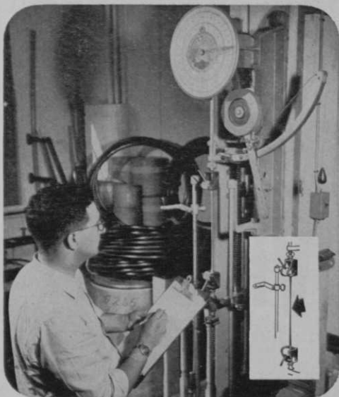
(Above) Impact test. Before approval can be given to production, raw material is tested for satisfactory resistance to impact. (Right) Tensile strength test. Virgin polyethylene is stretched to its limit to make sure Triangle Plastic Pipe will have more than its guaranteed working pressure.
