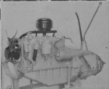
Here's a closeup of the thoroughly efficient, reliable and economical Ford Model 40, four cylinder tractor engine with a heavy-duty, four-speed transmission. Users report that five to six gallons of gas a day is all that is required—a saving for you.
