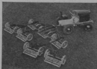
This fast and flexible 7-gang combination cutting a 16-foot swath is, we believe, the most efficient and economical mowing outfit in the world.
