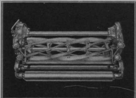
Eight-inch reel with double riveted spiders. Easy hand adjustment with positive locking. The Toro Trojan weighs 241 pounds net on the ground.
