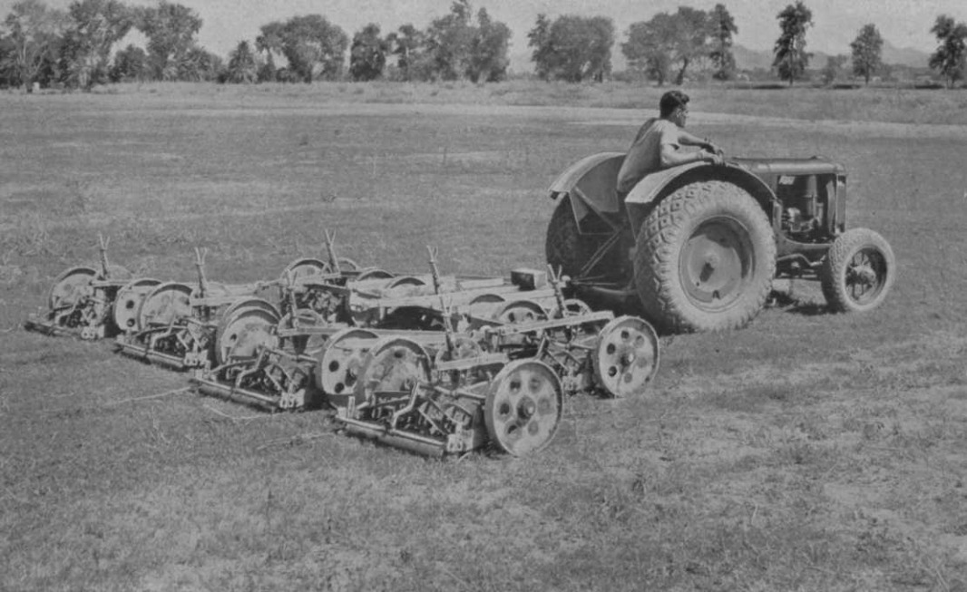
The International Fairway Tractor pulling the gang mowers on the new municipal golf course at Phoenix, Arizona.
