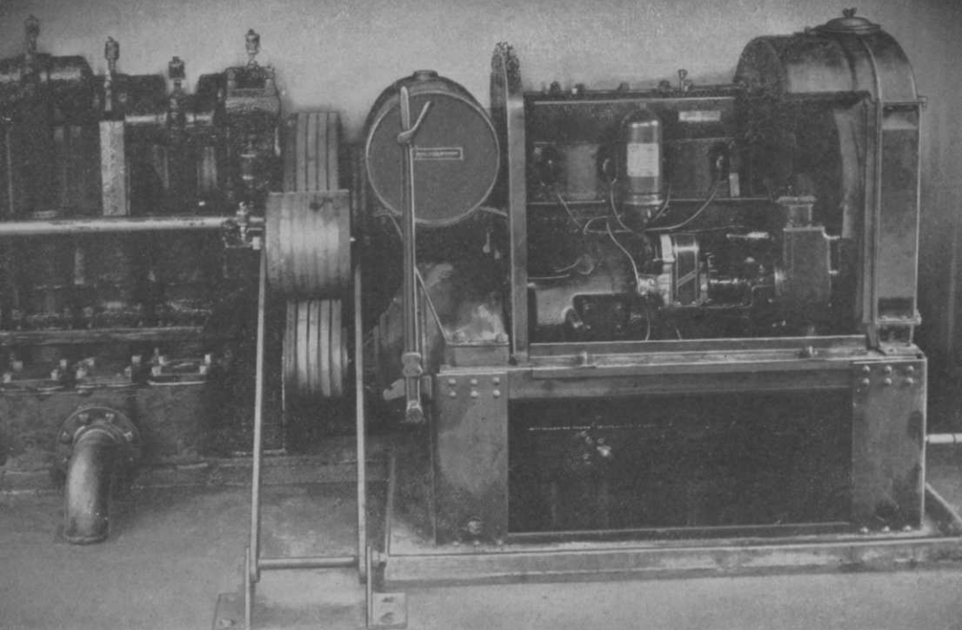
Installation of the International Power Unit and pump in the pump house at the Hamilton Golf & Country Club, Ltd., Ancaster, Canada.
