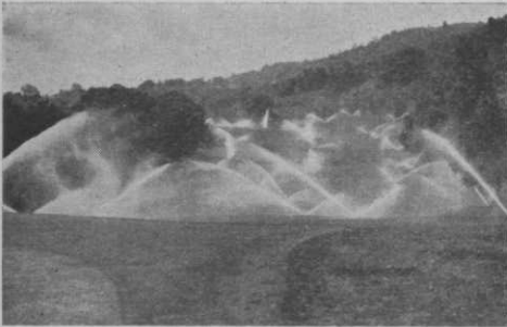
Castlewood Country Club, Pleasanton, California, showing the most modern irrigation system in the world—fairways, greens, tees, lawn area.
