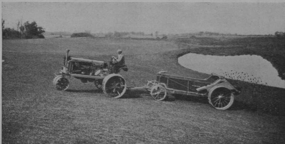
McCormick-Deering Fairway Tractor and Manure Spreader in Action
