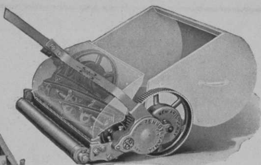
New Aristocrat, 19-inch cut. Weight 58 lbs. Price in Phila. ....$40.00 Grass Box, Extra ..... 8.00
