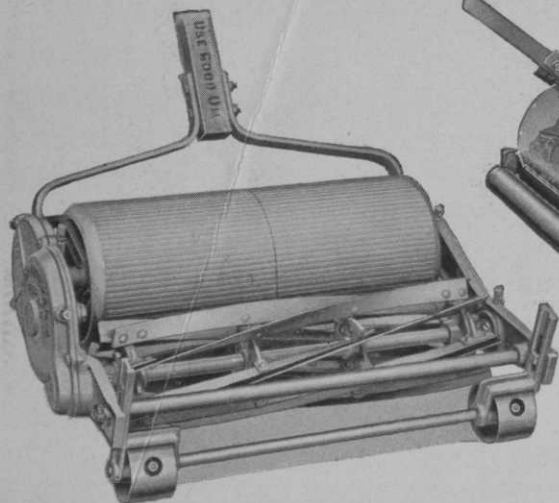
Super Roller Mower, 18-inch cut. Weight 58 lbs. Price in Phila. ....$50.00 Grass Box, Extra ..... 8.00 Carriage, Extra ..... 5.00
