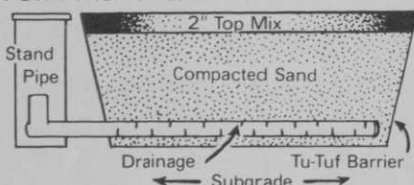
PURR-Wick Cross Section
