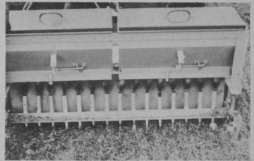
Seed is tubed into the soil after mat has been sliced away
