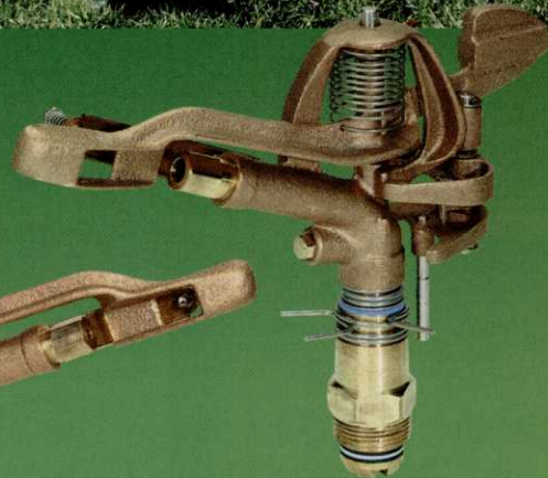
1" Flow: 15-45 GPM Spacing: 50-80 ft.
