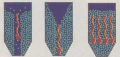
Ratholing Severe Funnel Flow Uniform Flow
