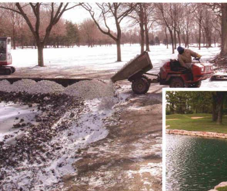
Landscape fabric is covered by crushed stone on the bank of the drained pond.
