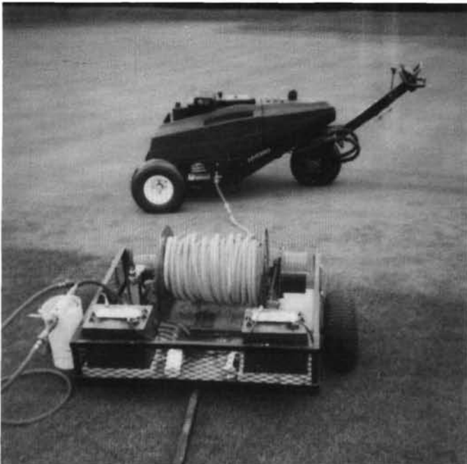
Trailer showing the 2 batteries, and a filter hook-up for the incoming water to the HydroJect 3000.
