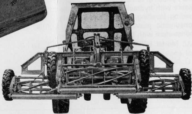
GREENS HY-RANGER GREENS RANGER TRAILED GANG MOWERS GREENS VERGE MASTER 30"
