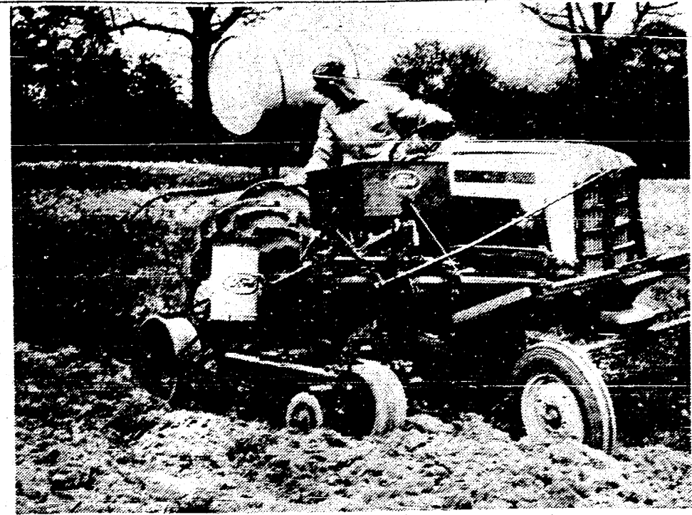
ONE PASS OVER FIELD REPLACES FOUR: The ground is plowed and seeds are planted, fertilized and sprayed all in one operation with this experimental rig, under development at Michigan State and Cornell Universities since 1951. The "plow-plant" system for row crops uses existing farm implements and one new piece of equipment, a special one-row planter soon to be commercially available.
