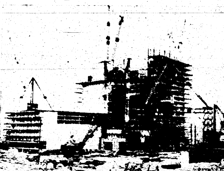
THIS IS ONE of two atomic piles at Calder Hall power station in England. It is the first step in Britain's 10-year atomic power program.
