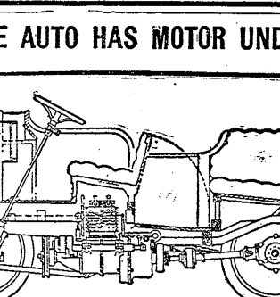
By placing the Air-Cooled Engine Under the Front Seat, This Automobile, of Japanese Design, Secures a Large Seating Space in a Light Car.
