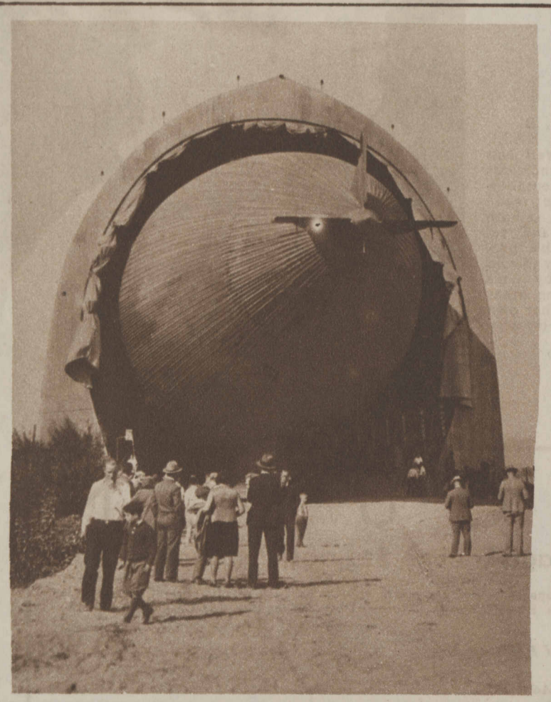
POISED FOR ITS FIRST FLIGHT —Capt. Thomas W. Slate's all-metal dirigible, City of Glendale, has been completed at the California city of that name. Among its new features of design is the placing of the engine in the nose, where it furnishes power to create a vacuum ahead of the ship. (Photograph from Pacific and Atlantic.)
