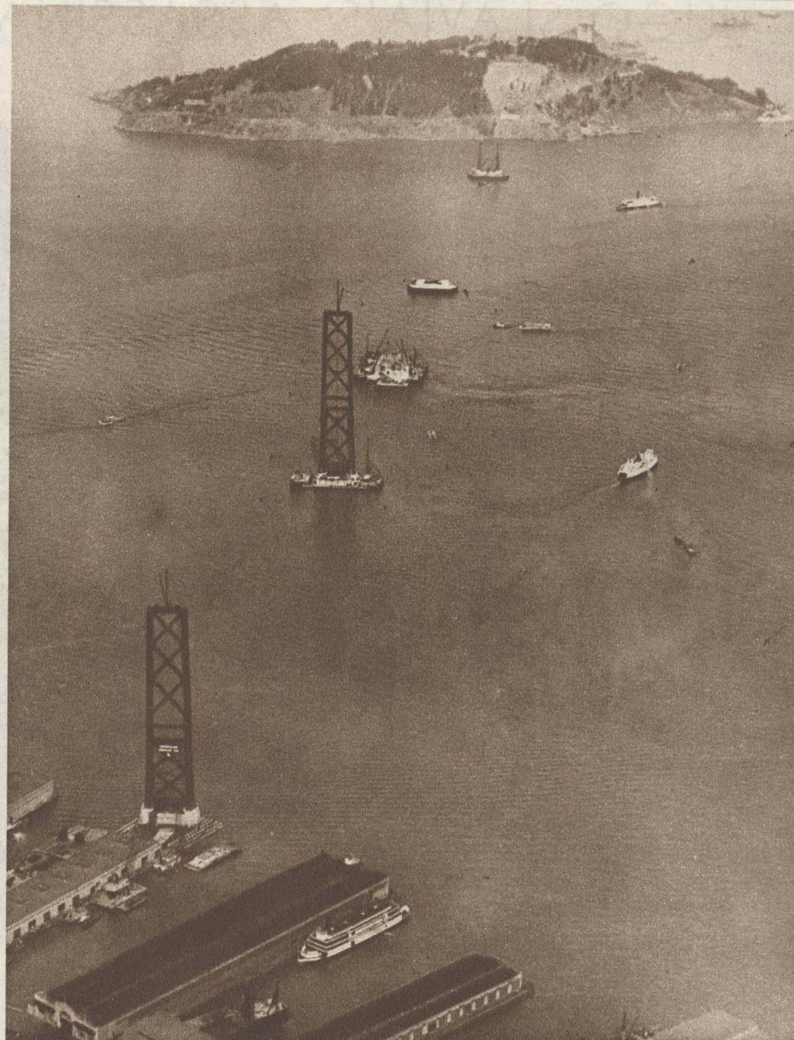
TOWERS of the Oakland-San Francisco bridge near completion. (Acme photo.)
