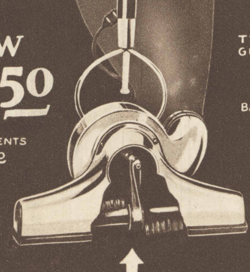
CUT AWAY VIEW SHOWING MOTOR DRIVEN BEATING BRUSH
