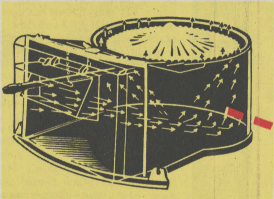
DRAFT AIR PREHEATED MAKES FIRE BURN BETTER
