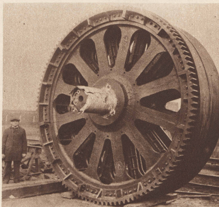
37 TONS OF PULLEY —A 13 foot fabrication from Gary which will form part of the machinery of the new railroad bridge across the Des Plaines at Joliet. The new span was necessitated by the Illinois waterway project.
