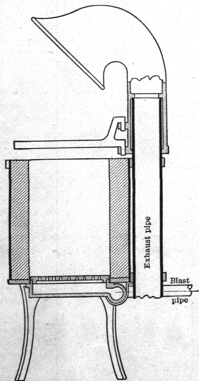
TEMPERING FORGE.
