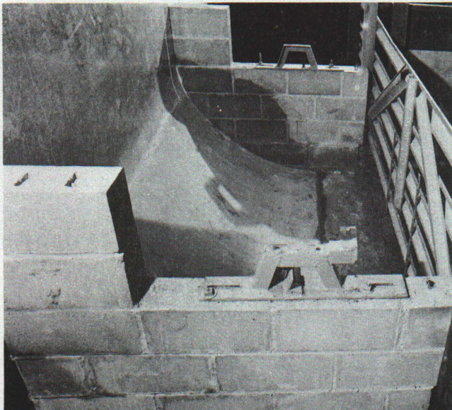
Fig. 3. It is difficult to pour a curved concrete spillway higher than 30" to 36". Extend the spillway upward with a thin piece of sheet metal and caulk where it overlaps the concrete.
