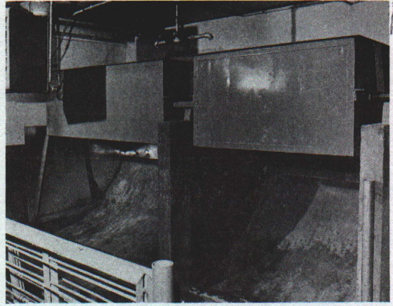
Fig. 2. Tanks can be mounted on a steel frame, poured concrete wall or a 6" concrete block wall. Likewise, the curved spillway can be constructed of concrete or metal. Use the material that fits your capabilities best.
