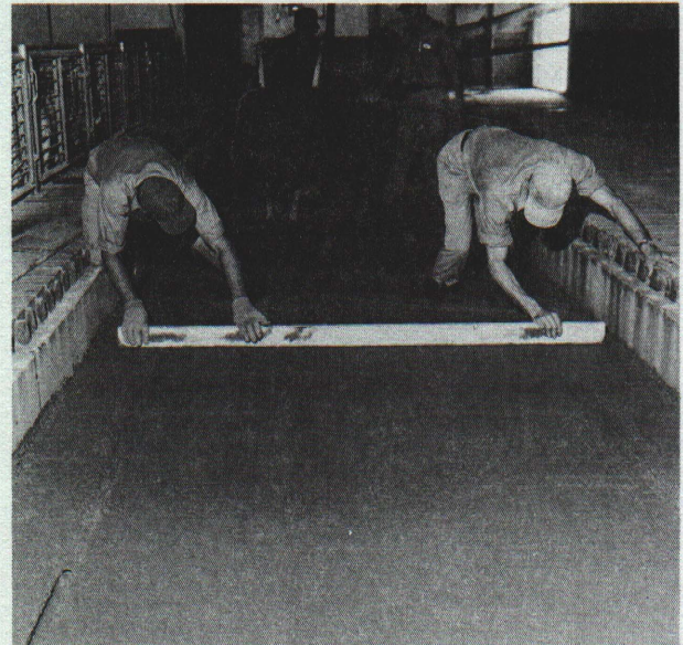
Fig. 6. Skirting concrete on two 1" pipes resting on the 2" x 4" stakes. Since the pipes have an outside diameter of 1 \frac{1}{4} ", the length of the stakes must be reduced by this amount to give the desired floor elevation.
