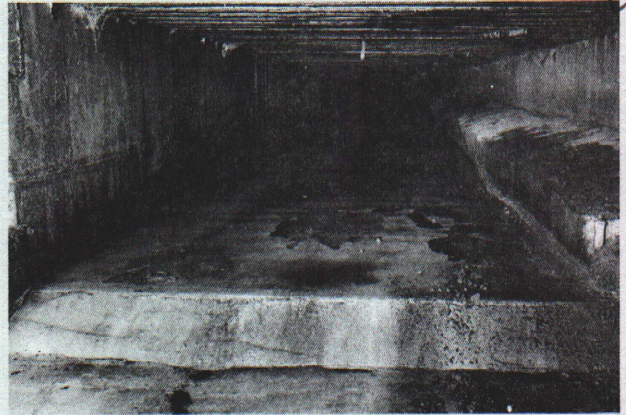
Fig. 9. Before (left) and after (right) flushing. The raised surface (right in both photos) is directly under the center alley of a completely slotted floor. A row of concrete blocks laid the length of the trench and capped to form a sloped surface permits the alley to be hosed off as needed. By narrowing the trench, the flush water is confined to the manure area and less water is required.
