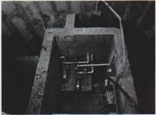
Fig. 8. These two pumps are used to recycle water from a lagoon back into the building for flushing or to pump water for irrigation. The water is taken 4' off the bottom of the lagoon and passed through a screen before reaching the pump.
