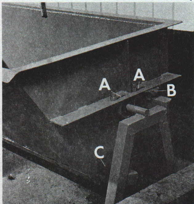
Fig. 1. Two methods of mounting bearings are illustrated in these pictures. Both are equally satisfactory. A 3 1/2" diameter hard rubber bottle stopper makes an ideal bumper. Rubber acts as a shock absorber and eliminates the noise caused by the tank dumping.
