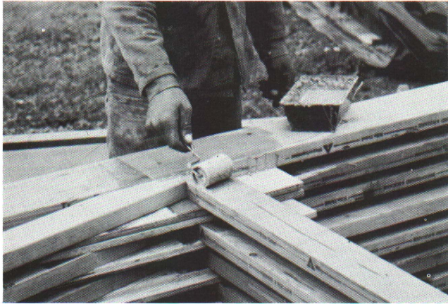
Figure 7—Applying glue with a paint roller. A paint brush can also be used.
