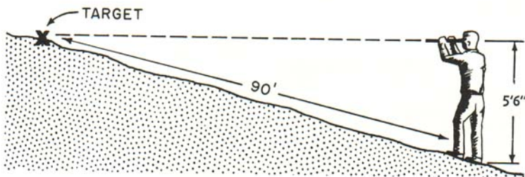
Fig. 4.—In this sketch, percent slope is being estimated with a hand level. The man has established that his eye or line of sight is 5.5 feet above the ground when he stands erect. He sights uphill through the level to an object which he has placed on the ground
