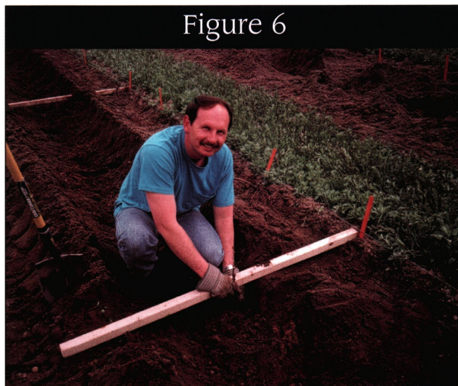
Figure 6 – A trench was opened for planting a row of grapevines. A tensioned wire offset 30 inches from the row of vines is used to place the vine precisely in the trench. The measuring stick is 60 inches long with a mark for vine placement in the middle of the stick.
