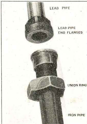
Figure 9: Lead pipe can be attached to iron pipe by an ordinary union.
