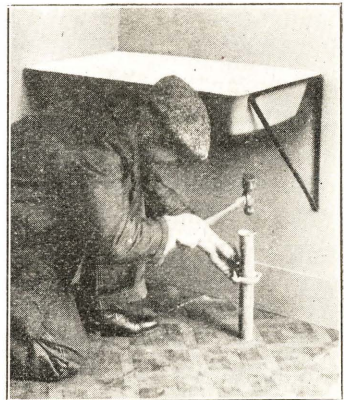
Figure 7: Lead pipe should be flanged to fit the pipe clamp.
