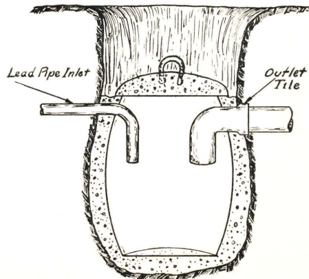
Figure 12: A grease trap made with a barrel used as a form.
