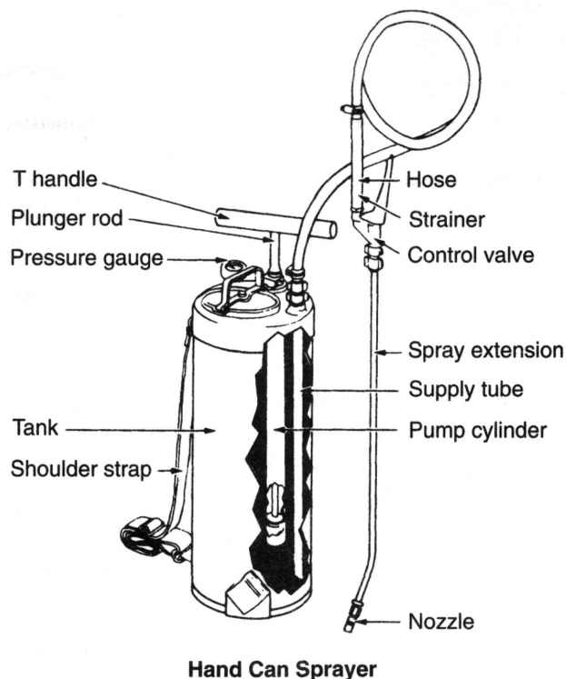
Hand Can Sprayer
