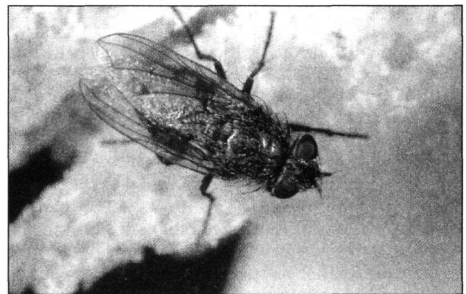
House Fly
