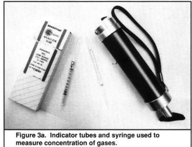
Figure 3. Measuring gas concentration.
