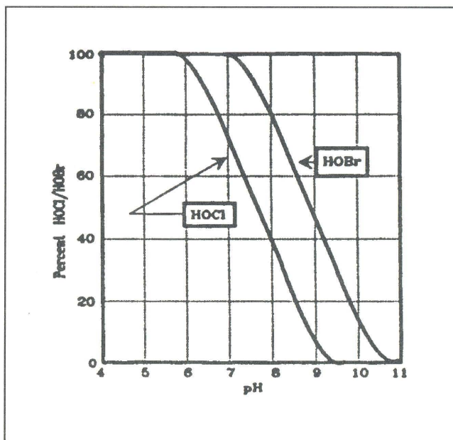
Figure 3-1. Effect of pH on the active forms of HOCl and HOBr.
