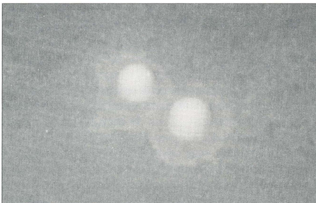
Improper application of biocide tablets. Tablets of formulated biocides should be metered and fed, or suspended in the systems water flow rather than dropped in the basin as shown here. Note the dark pock marks in the concrete surface damaged by previous applications.
