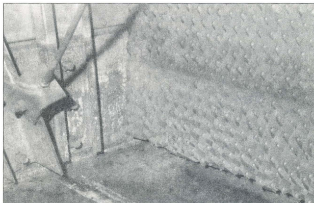
Two examples of cooling tower 'fill' through which water circulates.
