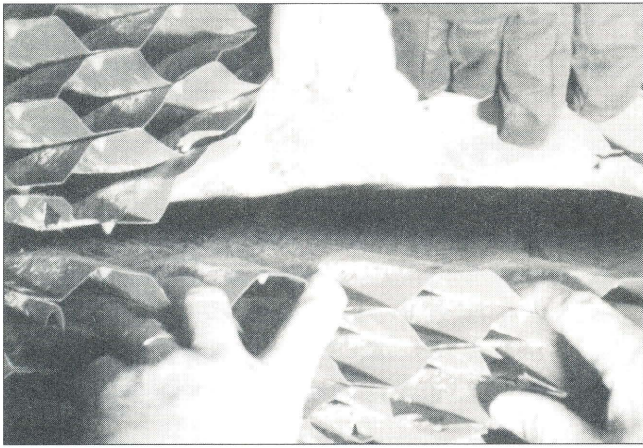
Close-up of cooling tower fill where microbial growths can accumulate and reduce system efficiency.
