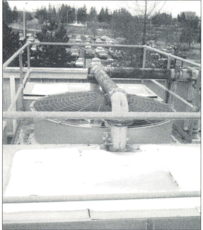
Removable sunlight covers on distribution decks are used to minimize algae growth. (Winter photo shows snow on covers.)
