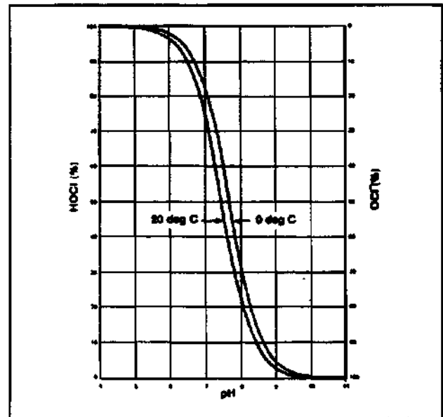
Figure 3-1. Relationship between HOCl, and OCl - , and pH.
