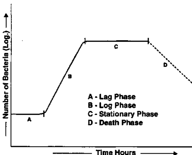
Figure 2-4. Typical growth curve of microorganisms.
