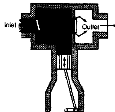
Piston pump.
