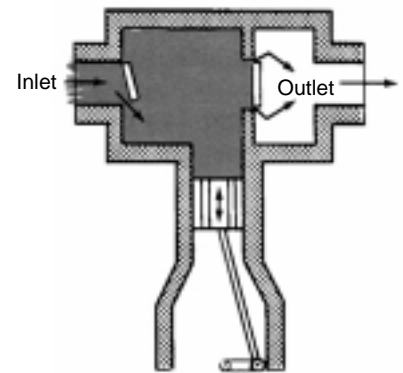
Piston pump.
