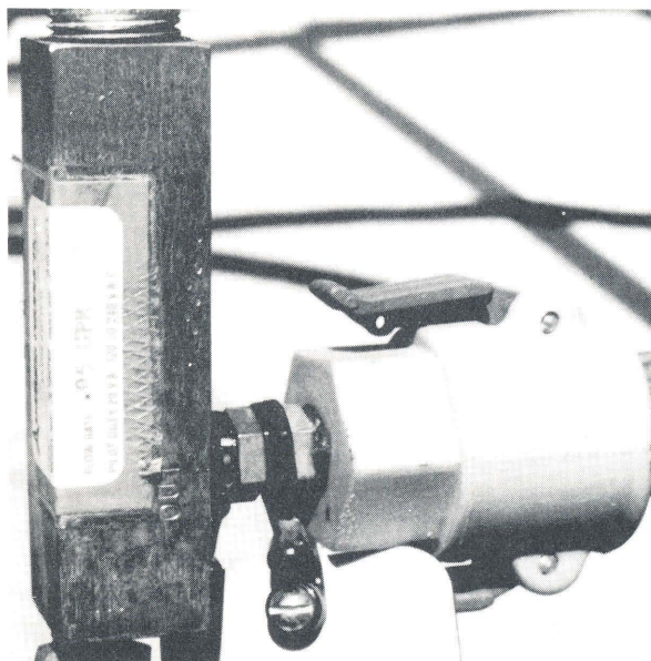
A flow sensor on the chemical injection line can shut down the irrigation system and pumping plant if chemical flow stops.
