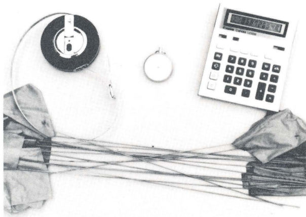
Tape, stopwatch, calculator and flags are needed in the calibration process.
