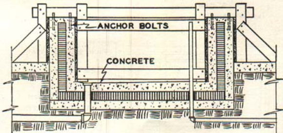
Fig. 9. Step No. 5. Concrete is first placed on the floor to the height of the side forms, then the wall space is filled on either side of the insulation. Anchor bolts should be placed in the top of the concrete wall for attaching the plate. The nuts of the bolts should be countersunk below the top of the plate.
