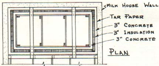
Fig. 6. Another method of setting inside and outside forms for the concrete tank. Note the insulation in place before the concrete is poured.
