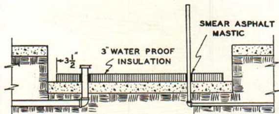
Fig. 3. Step No. 2. Here the 3" water-proof package insulation has been placed on the cement floor. Note that a 3\frac{1}{2} " space is left all around the insulation for the concrete wall. The insulation should be arranged as shown in Fig. 4 (below).
