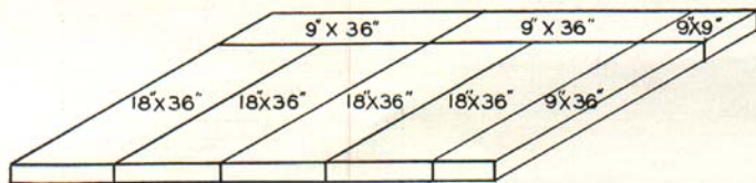
Fig. 4. Method of arranging the insulation packages for the floor of a four-can tank.
