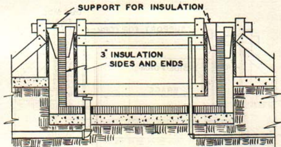
Fig. 7. Step No. 4. The package insulation is placed in the center of the wall space and held in place by the wedges at the top. See details for arranging insulation in Fig. 8 (below).
