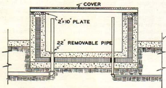
Fig. 10. Step No. 6. The cover attached by hinges to plate.
