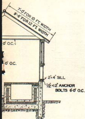
GABLE ROOF
