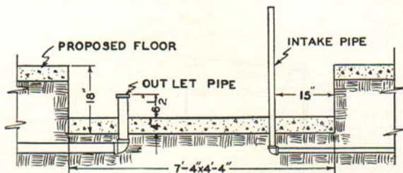
Fig. 2. Step No. 1 shows the excavation for the tank with the concrete sub-floor in place.
