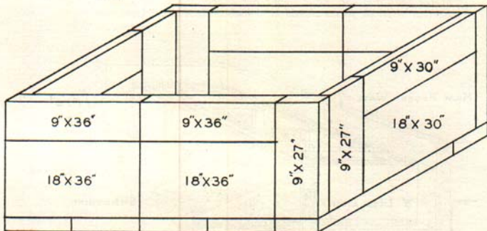
Fig. 8. Method of arranging the insulation for the side walls of a four-can tank.
