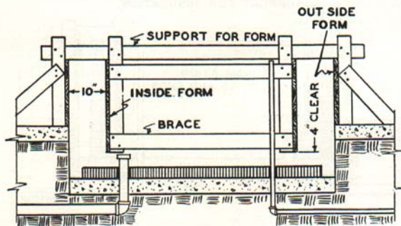
Fig. 5. Step No. 3. The outside forms have been placed for the wall of the tank and the inside forms are supported on the outside forms. Bottom of inside forms should be 4 inches above floor insulation.
