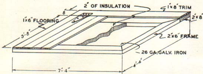
Fig. 11. Step No. 6 shows details of the construction of the cover.
