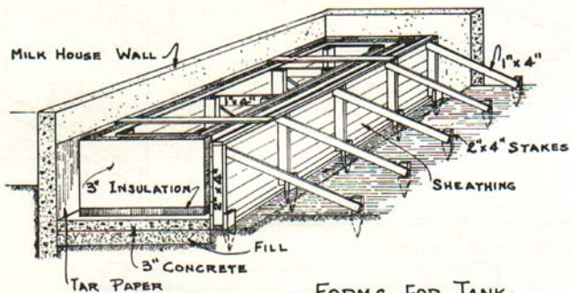
Fig. 5. Step No. 3. The outside forms have been placed for the wall of the tank and the inside forms are supported on the outside forms. Bottom of inside forms should be 4 inches above floor insulation.
