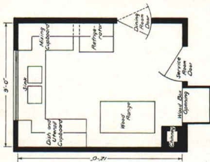
Fig. 25. U-arrangement. Small and compact.
