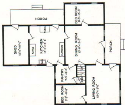
Fig. 31. Original house plan. Note the poorly arranged kitchen.
