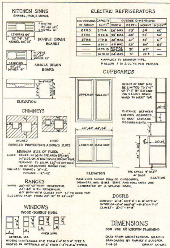
Fig. 34. Standard measurements.
