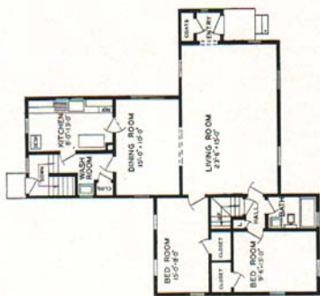
Fig. 32. The remodeled house plan of Fig. 31. Note the convenient kitchen arrangement.
