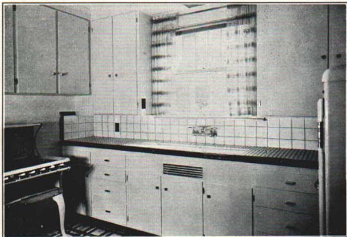
Fig. 21. A compact convenient kitchen arrangement. Notice these features: light in ceiling above sink, wall outlets for small electrical equipment, cupboards on wall space over the range, glazed tile working surface, double sink, ventilated cupboard below sink, and toe space at bottom of cupboard.
