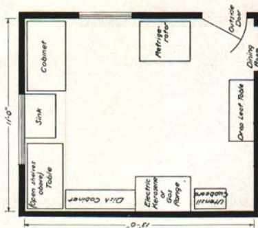
Fig. 30. A broken U-arrangement using portable equipment.
