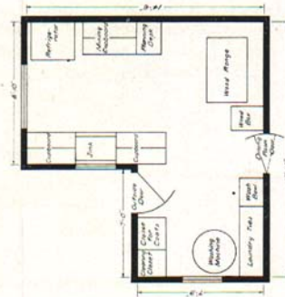
Fig. 29. Broken U-arrangement. Each center separate.
