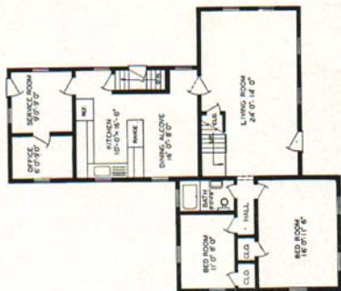
Fig. 33. Another remodeled house plan of Fig. 31. Note the convenient kitchen arrangement.
