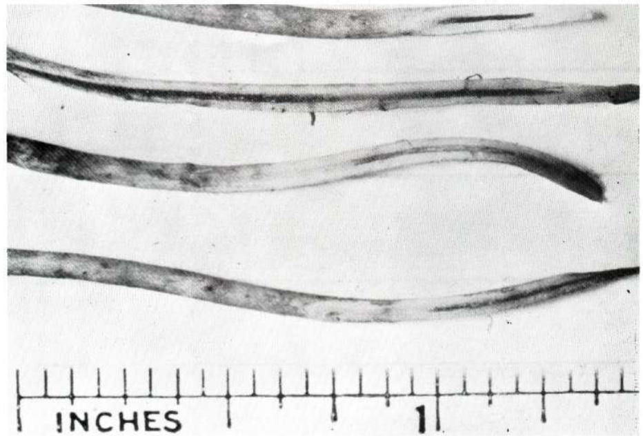
Fig. 3. Discolored root core (stele) resulting from red stele root rot.
